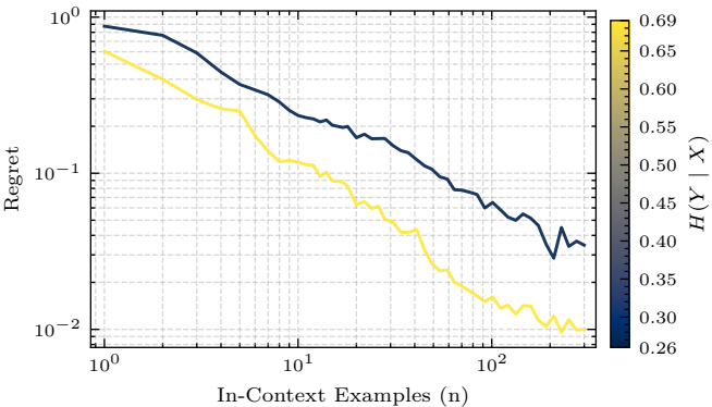
In-Context Learning Regret for Qwen-2.5 (3B)
